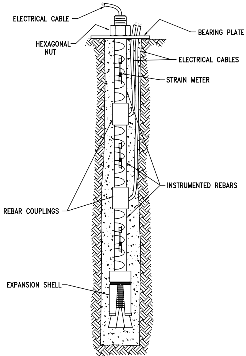
Figure 2: Multiple Instrumented Rebar System Typical Borehole installation
