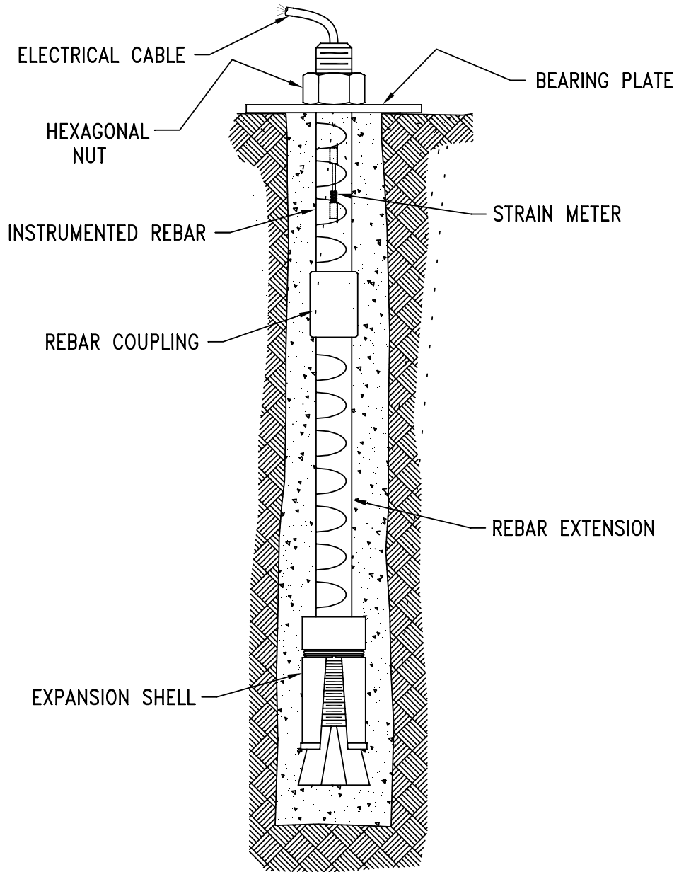
Figure 1: Single Point Instrumented Rebar Typical Borehole installation
