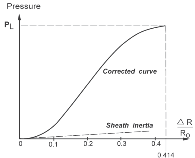
Example of pressuremeter test results
